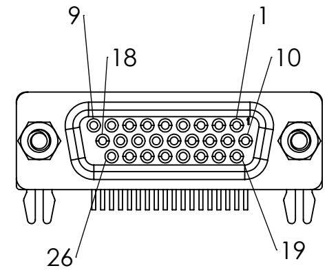
Connector Pinout (Female)
