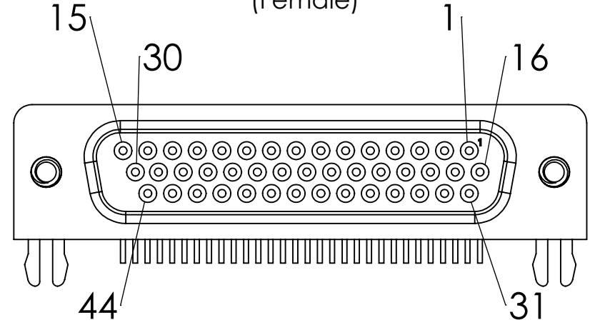
Connector Pinout (Female)
