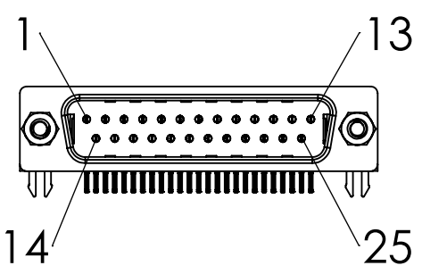
Connector Pinout (Male)
